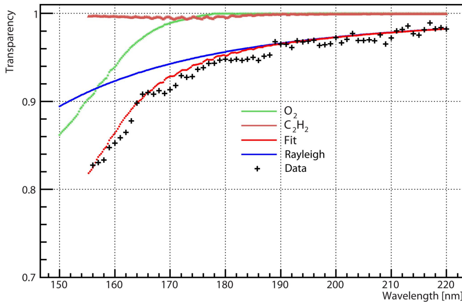
Figure 7. Typical example of a transparency curve for the C_4F_{10} of COMPASS RICH-1: the fitted transparency curve (in red) corresponds to contamination levels of O_2 = 2.3 ppm, H_2O = 0.0 ppm, C_2H_2 = 0.03 ppm.
