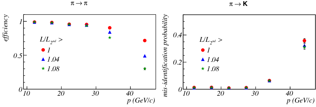
Figure 26. Efficiency and misidentification probability for \pi as function of momentum.
