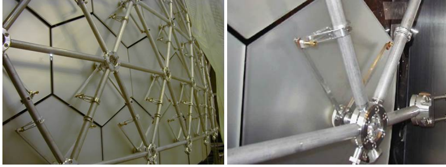
Figure 9. Picture of the back side of the mirrors and of the adjustment screws
