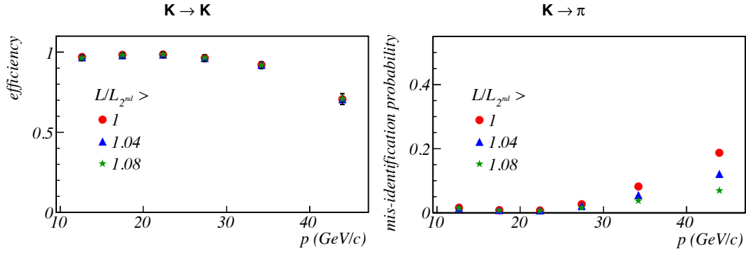
Figure 27. Efficiency and misidentification probability for K as function of momentum.
