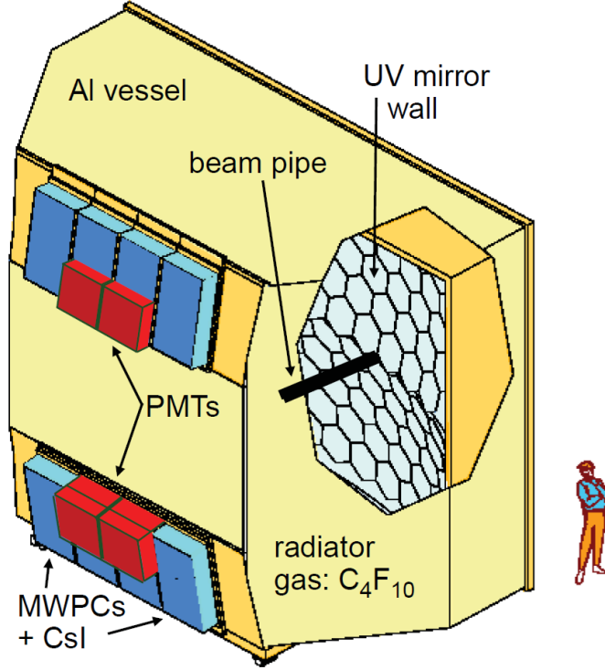
Figure 3. Artistic view of COMPASS RICH-1.
