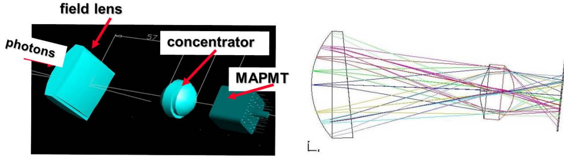
Figure 21. Artistic view and scheme of the individual fused silica lens telescope.
