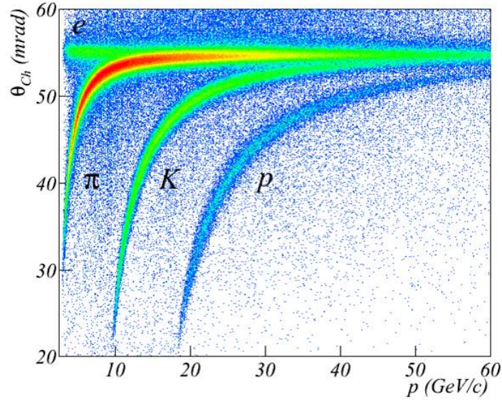
Figure 23. The measured ring Cherenkov angle versus particle momentum p .
