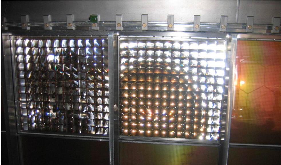
Figure 20. Two panels with lens telescopes and MAPMTs seen from inside of the RICH-1 vessel.
