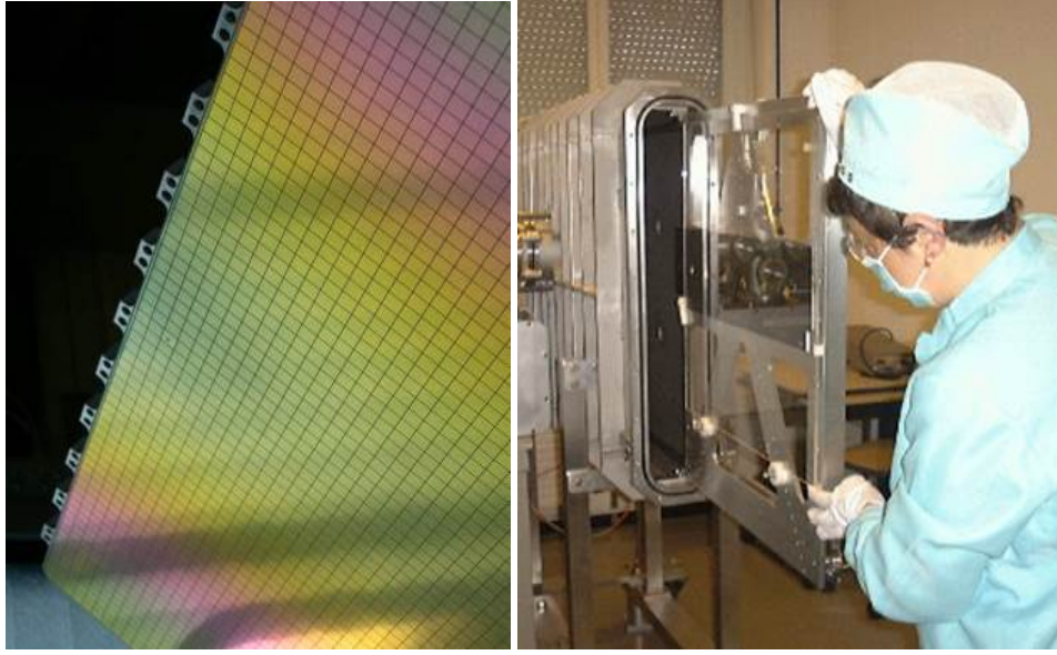
Figure 13. Picture of a CsI-coated photocathode and of a quartz window during the transparency measurement operation.
