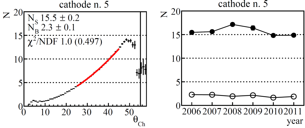
Figure 18. number of detected Cherenkov photons versus Cherenkov angle and variation over six years of the extrapolated number of detected Cherenkov photons for \theta_{Ch} = 55.2 mrad for the pions with a ring fully contained in one of the photocathodes (cathode n. 5).
