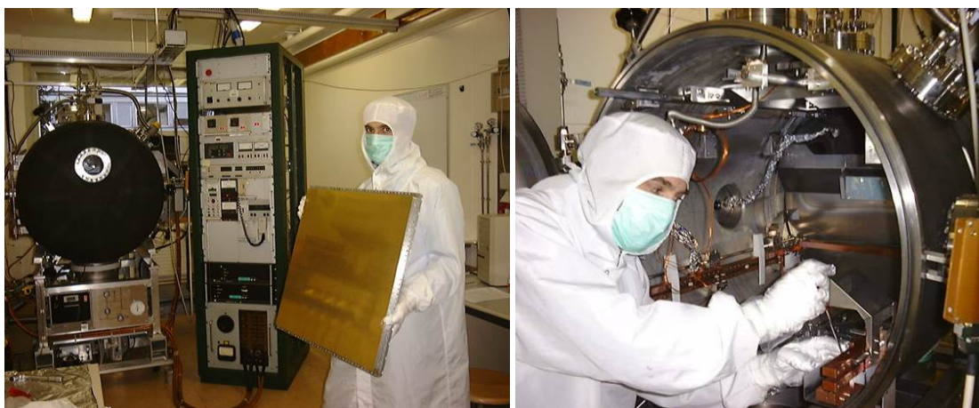
Figure 15. Pictures of the COMPASS photocathode and the CERN CsI evaporation plant.
