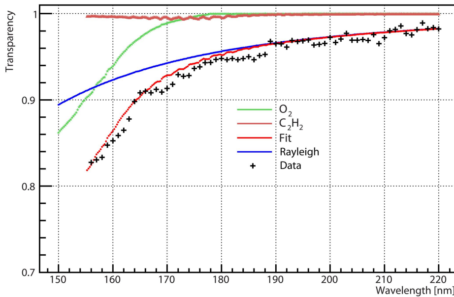
Figure 7. Typical example of a transparency curve for the C_4F_{10} of COMPASS RICH-1: the fitted transparency curve (in red) corresponds to contamination levels of O_2 = 2.3 \text{ ppm} , H_2O = 0.0 \text{ ppm} , C_2H_2 = 0.03 \text{ ppm} .
