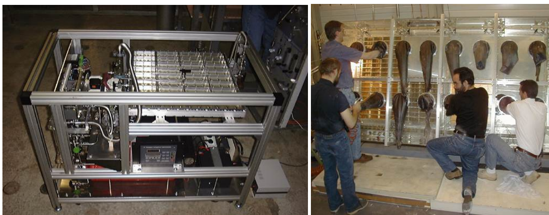
Figure 16. Pictures of the COMPASS photocathode transport system and of the the installation glove-box.
