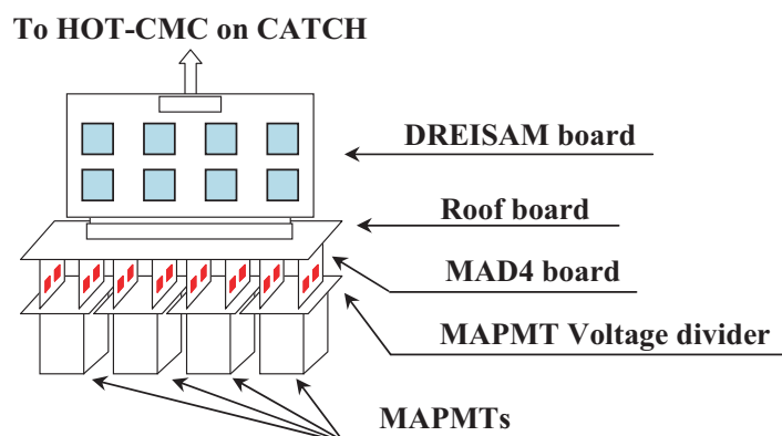
Fig. 2. Scheme of a basic read-out unit.
