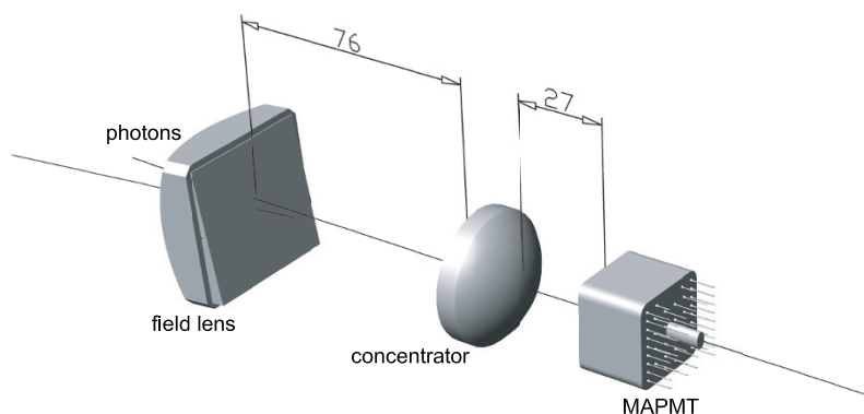
Fig. 1. Scheme of the two-lenses telescope system, measures being given in mm.
