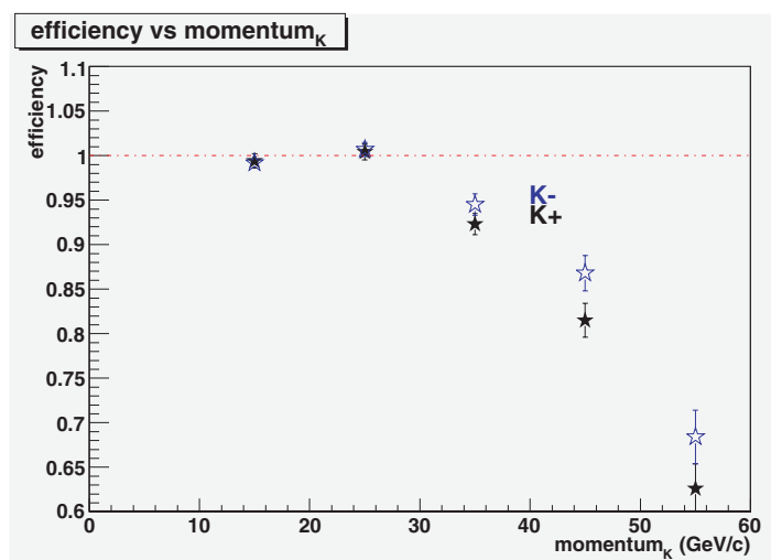
Fig. 9. Efficiency versus particle momenta (Kaons): for smaller Kaon momenta, the efficiency is 100%, whereas for higher momenta, the efficiency decreases due to the Cherenkov emission angle becoming practically equal for different particles at high momenta.
