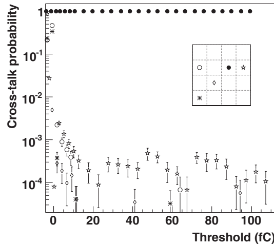
Fig. 6. Cross-talk measurement: hit rates of the illuminated reference pixel (closed circle) and in different neighbouring channels, each normalised to the reference pixel.
