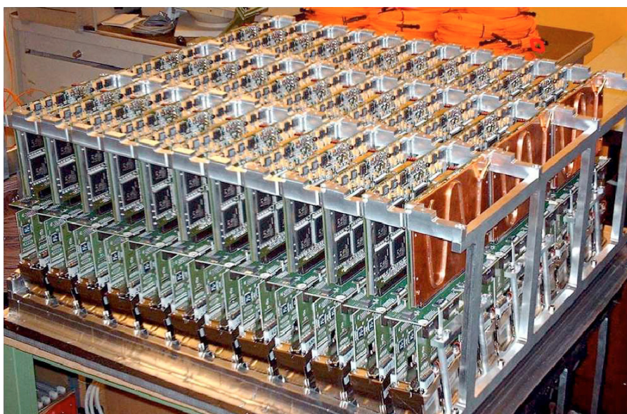
Fig. 3. First quadrant: one quadrant of the new detection system comprising 144 MAPMT, fully equipped with FE electronics. The FE cards are water-cooled by single waterline copper plates, as indicated by the three DREISAM boards in the front.
