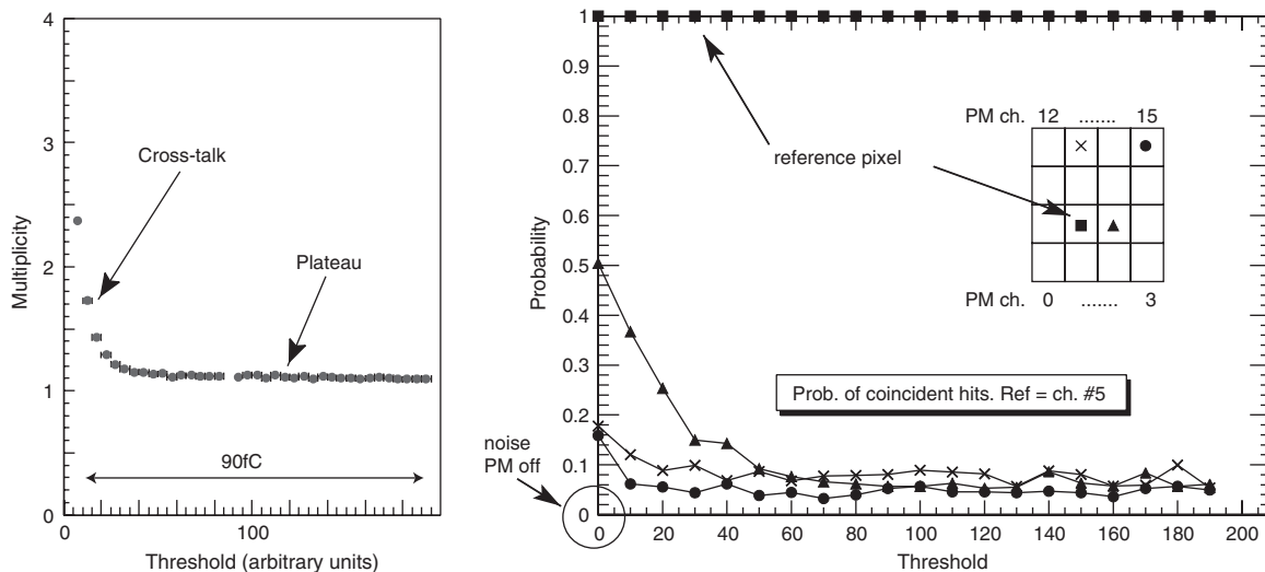
Fig. 2. Results from the 2004 test beam. The left picture shows the measured hit multiplicity for one of the MAPMTs at nominal HV, as a function of the applied electronics threshold. The horizontal scale is in arbitrary units, relative to the measured electronics noise. The right plot shows the measured cross-talk as a function of the discriminators threshold (arbitrary units) for some of the MAPMT pixels, when one of the central pixels is taken as reference.
