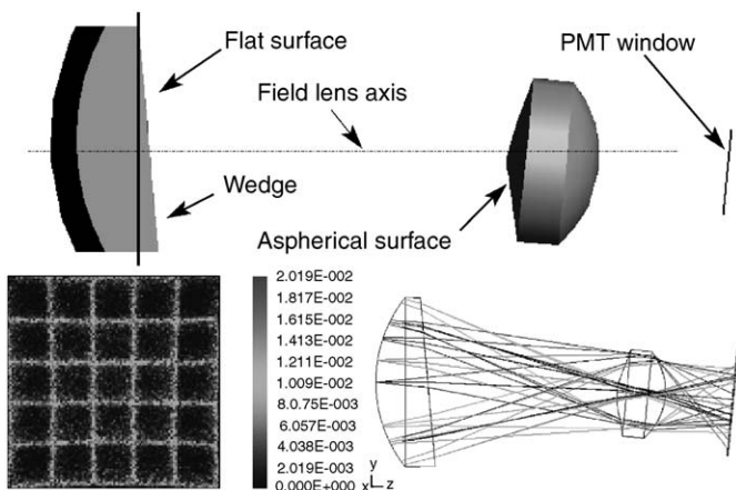
Fig. 3. Schematic view of the optics used to condense the Cherenkov photons on the MAPMT sensitive surface. The design comprises one aspherical element to reduce image distortion and aberration. The bottom pictures show the simulated response of the optics to incident rays with angles of \pm 8.3^\circ maximum.
