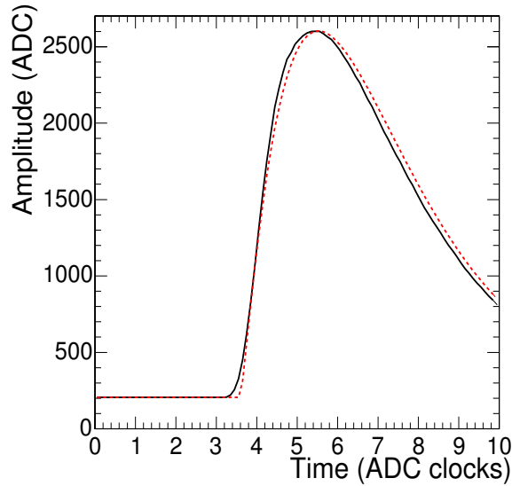
Figure 10: Signal pulses for a 120 GeV electron beam: the solid line shows the profile of the signal in the channel under study, and the dotted line shows the average representation of the signal.
