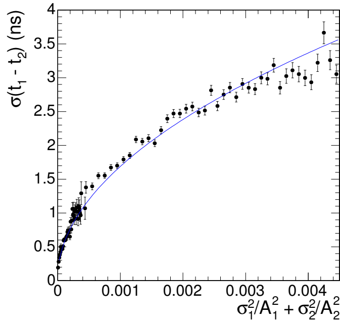
Figure 7: Resolution on time difference between two crystals 703 and 704 as a function of the sum of inverse square amplitudes. The fit is made assuming that the parameters a and b of Equation 4.1 are the same for both crystals.
