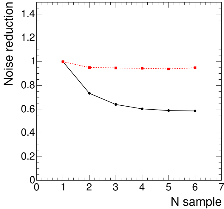
Figure 2: Expected noise reduction ( \sqrt{\sum w_i^2} ) as a function of the number of samples used for the reconstruction in the case of no noise correlations between time samples (solid line) and in the case of the correlations found in test beam data (dashed line).
