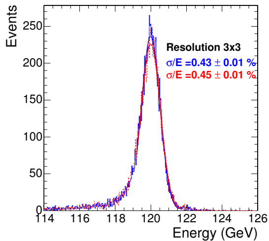
Figure 15: Distribution of the reconstructed amplitude summed in a 3 \times 3 matrix of crystals using pedestal-subtracting weights with (solid histogram, \sigma/E = 0.43\% ) and without (dashed histogram, \sigma/E = 0.45\% ) jitter compensation. (Asynchronous data using all phase bins).
