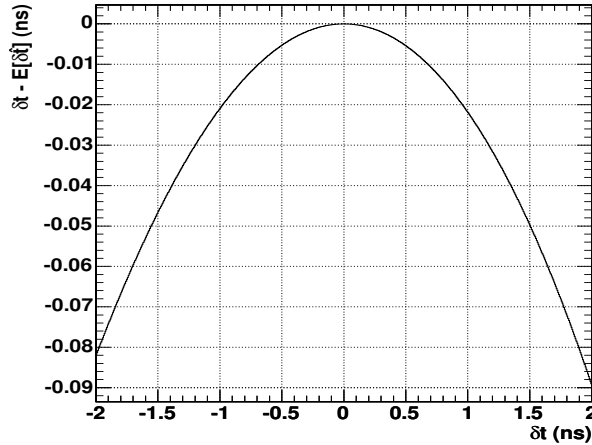
Figure 6: Time bias, \delta t - E[\delta t] , introduced by the linear approximation, as a function of \delta t .
