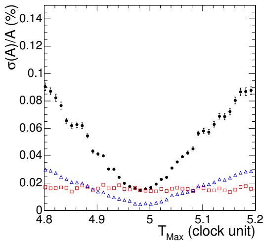
Figure 14: Amplitude measurement spread due to jitter as a function of pulse maximum time. Solid circles and open squares correspond to simulated events with a timing jitter of 0.65 ns. The solid circles are obtained when standard amplitude reconstruction is used, whereas the open squares result from use of jitter-compensating weights. The open triangles correspond to standard amplitude reconstruction when the jitter is equal to 0.2 ns as expected in CMS.
