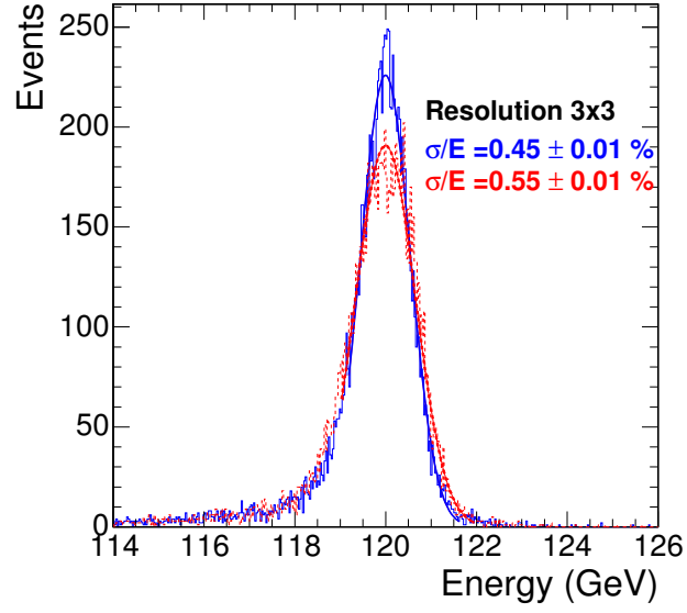
Figure 12: Distribution of the reconstructed amplitude in a 3 \times 3 matrix for a 120 GeV beam using the weights derived from an average representation of the signal pulse (dashed histogram) and the true profile of the signal in the crystal studied (solid histogram). Truncated Gaussian fits are superimposed on both distributions and are used to derive the energy resolution: dashed histogram 0.55%, solid histogram 0.45%. (Asynchronous data using all phase bins).
