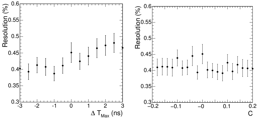
Figure 5: (Left) Energy resolution in a 3×3 matrix of crystals measured with a 120 GeV electron beam, as a function of \Delta T_{\text{Max}} . (Right) Energy resolution as a function of the contraction factor, C .
