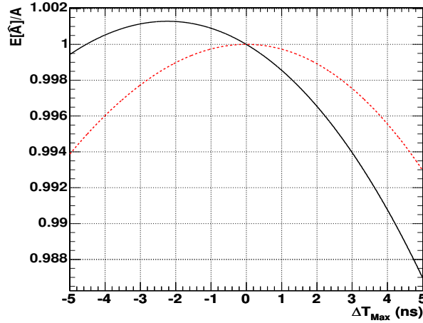
Figure 4: Reconstructed amplitude over true amplitude, E[\hat{A}]/A , as a function of timing difference \Delta T_{\text{Max}} . The solid line shows the value obtained with 3+5 pedestal-subtracting weights, and the dashed line shows the value obtained using 3+1 pedestal-subtracting weights.
