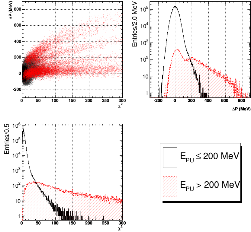
Figure 9: Distribution of \Delta P versus \chi^2 in ECAL barrel, together the projections of these variable plotted as histograms. Distributions are shown separately for pulses which include out of time pileup particles with an energy greater than 200 MeV and those which do not. The bands in the scatter plot correspond to particles from different bunch crossings.
