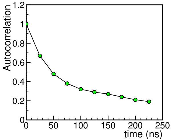
Figure 3: Measurements of the autocorrelation function at intervals of 25 ns, obtained from the top row of the normalized covariance matrix, averaged for six channels. The lines joining the points are intended to guide the eye.
