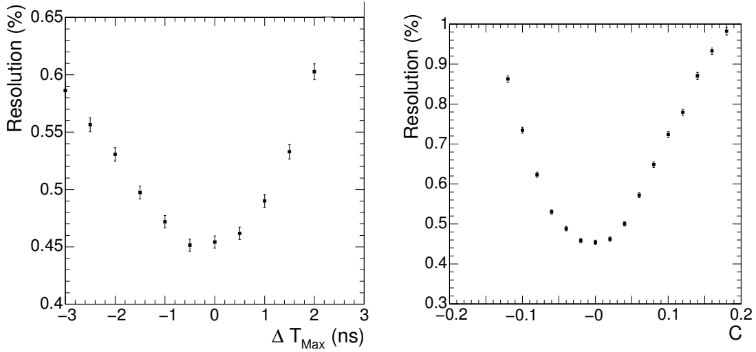
Figure 13: (Left) Energy resolution in a 3 \times 3 matrix of crystals for a 120 GeV electron beam, as a function of \Delta T_{\text{Max}} . (Right) Energy resolution as a function of the contraction factor, C .
