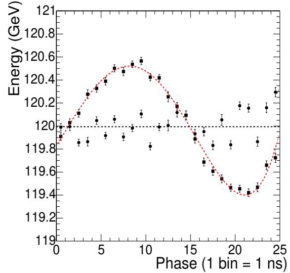
Figure 11: Average reconstructed amplitude summed in a 3 \times 3 matrix of crystals as a function of the phase using weights obtained with the average representation of the signal (squares) and the signal profile from the channel under study (circles). The polynomial fit and straight line are shown to guide the eye.
