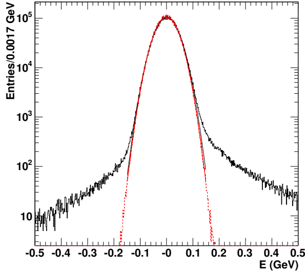
Figure 8: Reconstructed amplitude in ECAL barrel channels in the absence of a signal, without pileup (dashed histogram) and with pileup (solid histogram). A Gaussian of width 40 MeV is superimposed on the dashed histogram.
