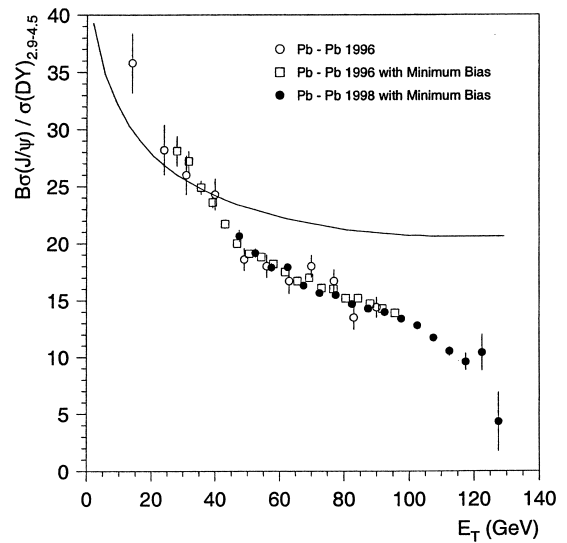
Fig. 4. \sigma_{\psi}/\sigma_{DY} ratio as a function of E_T , obtained with the standard and minimum bias analyses of the 1996 and 1998 data samples. The curve represents the J/\psi suppression due to ordinary nuclear absorption.
