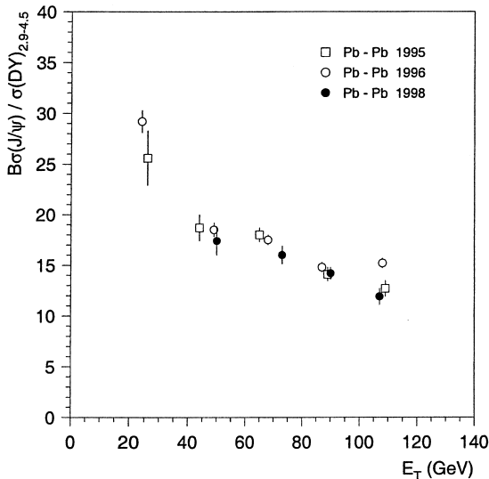
Fig. 3. \sigma_{\psi}/\sigma_{DY} ratio as a function of E_T , obtained with the standard analysis of the 1995, 1996 and 1998 data samples.
