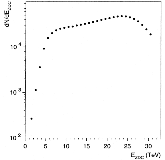
Fig. 2. E_{\text{ZDC}} spectrum measured in 1998 with the minimum bias trigger. The data are not corrected for the efficiency of the target algorithm and the contribution from secondary particles has not been subtracted.
