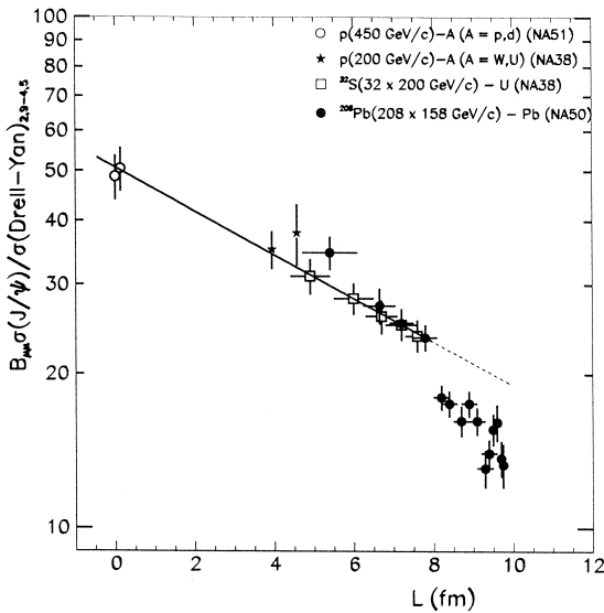
Fig. 6. Ratios of the J/\psi to Drell-Yan cross-sections as a function of the mean nuclear path length L , for NA38, NA50 and NA51 data. The NA38 and NA51 data are rescaled to 158 GeV/c. The line corresponds to the simple exponential fit with \sigma_{\text{abs}} = 5.8 mb.
