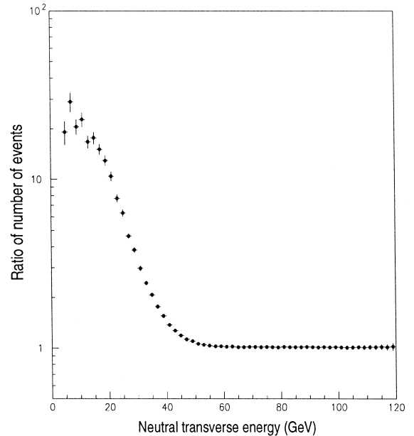
Fig. 2. Ratio of the number of events selected by the contour-cut method and by the target algorithm.
