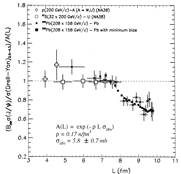
Fig. 9. The \sigma_{J/\psi} / \sigma_{DY} ratios divided by the normal nuclear absorption suppression inferred from the NA38 and NA51 results.
