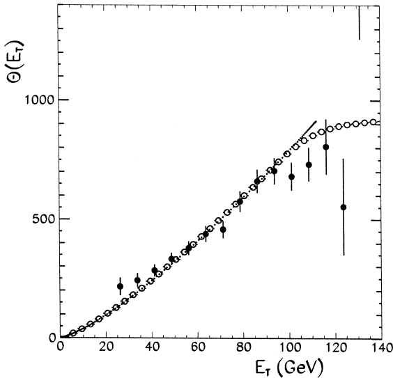
Fig. 7. The ratio \Theta(E_T) of Drell-Yan to minimum bias theoretical E_T distributions (open circles). Also shown is the corresponding ratio for the data (closed circles) and the calculated number of elementary nucleon-nucleon collisions (dotted line).
