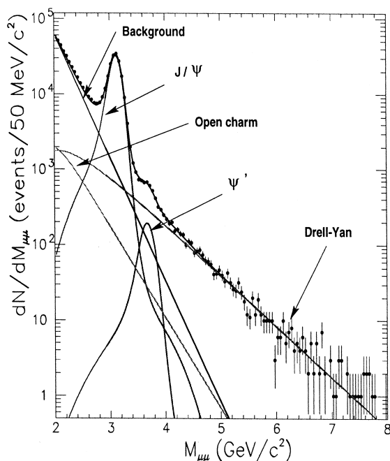
Fig. 3. Opposite-sign muon pair invariant mass spectrum for Pb-Pb collisions at 158 \text{ GeV}/c incident momentum.
