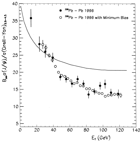
Fig. 8. Comparison of the ratios \sigma_{J/\psi} / \sigma_{DY} and \sigma_{J/\psi} / \sigma_{DY}^* based respectively on Drell-Yan and minimum bias events. The curve shows the same ratio for normal nuclear absorption, as plotted in Fig. 5.
