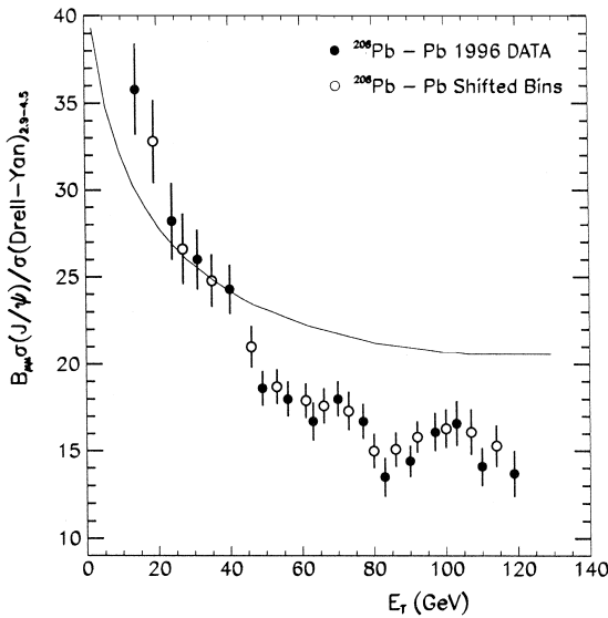
Fig. 5. Ratios of J/\psi to Drell-Yan cross-sections as a function of centrality in Pb-Pb collisions at 158 GeV/c. The line corresponds to the fit to lighter interacting nuclei shown in Fig. 6. It is supposed to account for ordinary nuclear absorption (see text) with \sigma_{\text{abs}} = 6.4 mb.
