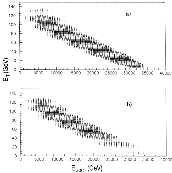
Fig. 1. Correlation between neutral transverse energy and very forward hadronic energy for J/\psi events using the new selection procedure with (b) and without (a) requiring the vertex identification by the target algorithm.
