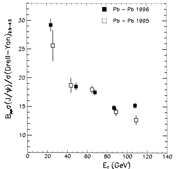
Fig. 4. The standard \sigma_{J/\psi}/\sigma_{\text{DY}} ratios for the 1995 and the 1996 data samples. The difference at the upper end of the E_T range is probably due to re-interactions in the target. See the text for details.
