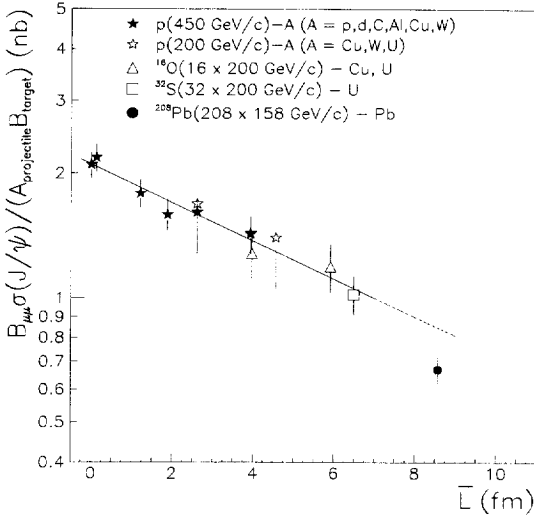
Fig. 3. The J/\psi “cross-sections per nucleon-nucleon collision” as a function of \bar{L} . The results obtained at 450 GeV/c and the Pb-Pb cross-section are rescaled as explained in the text.
