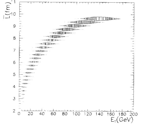
Fig. 4. Correlation between E_T and \bar{L} calculated for Pb-Pb collisions at 158 GeV/c for Drell-Yan events.
