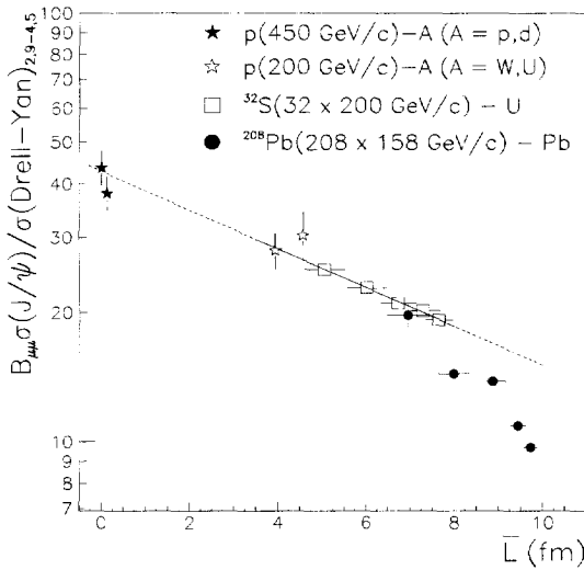
Fig. 5. The ratio of J/\psi to Drell-Yan cross-sections as a function of \bar{L} .
