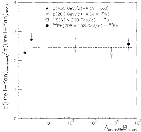
Fig. 1. The Drell-Yan K-factor as a function of the product AB of the projectile and target atomic mass numbers. The dashed line shows the average value of the data.
