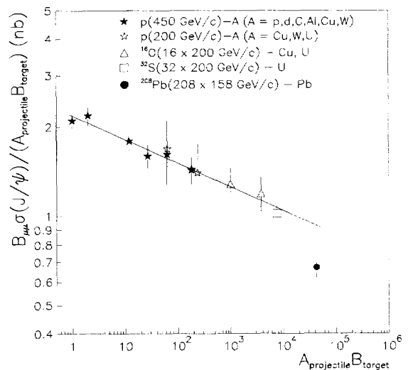
Fig. 2. The J/\psi “cross-section per nucleon-nucleon collision” as a function of the product AB of the projectile and target atomic mass numbers. The results obtained at 450 GeV/c and the Pb-Pb cross-section are rescaled as explained in the text.
