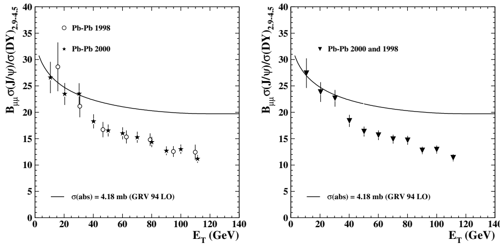
Fig. 10. Comparison between 1998 and 2000 results: separate (J/\psi)/\text{Drell-Yan} cross-sections ratios from 1998 and 2000 (left) and weighted average (right), as a function of transverse energy
