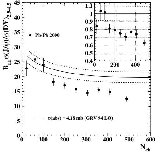
Fig. 6. The (J/\psi) / Drell-Yan cross-sections ratio as a function of charged multiplicity for the Pb-Pb 2000 data sample. The inset shows the ratio Measured/Expected, i.e. data over normal nuclear absorption
