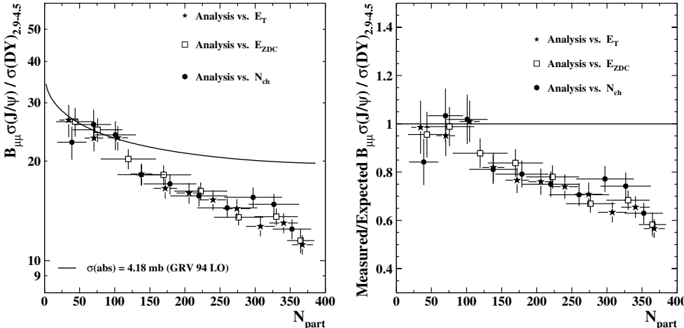
Fig. 7. The (J/\psi) / Drell-Yan cross-sections ratio as a function of N_{\text{part}} for three analyses of the Pb-Pb 2000 data sample, compared to (left) and divided by (right) the normal nuclear absorption pattern
