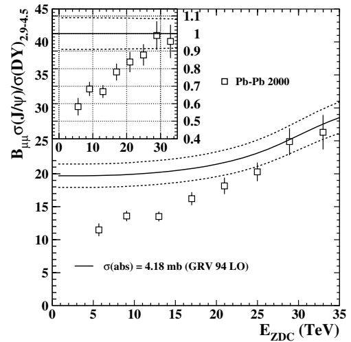
Fig. 5. The (J/\psi) / \text{Drell-Yan} cross-sections ratio as a function of forward energy for the Pb-Pb 2000 data sample. The inset shows the ratio Measured/Expected, i.e. data over normal nuclear absorption
