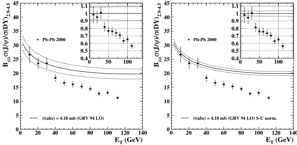
Fig. 4. The (J/\psi) / \text{Drell-Yan} cross-sections ratio as a function of transverse energy for the Pb-Pb 2000 data sample (left). The normal absorption curve is presented together with the combined error from the Glauber fit and the rescaling procedure (dashed curves). The inset shows the ratio Measured/Expected, i.e. data over normal nuclear absorption. The right panel presents the same data compared to the absorption curve computed using also S-U NA38 data for \sigma_{\text{abs}} determination and curve normalization
