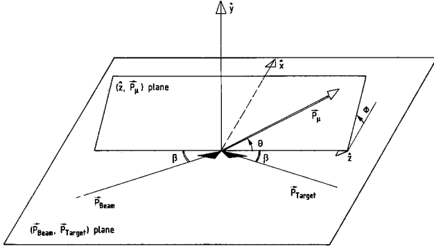
Fig. 2. Definition of the angles \theta and \phi in the center-of-mass system of the dimuon. The reference frame shown here is the Collins-Soper frame
