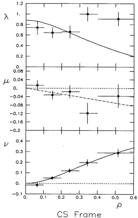
Fig. 7. Coefficients \lambda , \mu , and \nu as a function of \rho in the CS frame. The horizontal bars give the size of each interval. For \mu , the dot-dashed line is the result of the fit to (9); for \nu , the solid line is the result of the fit to (24), and for \lambda it is given by (15)
