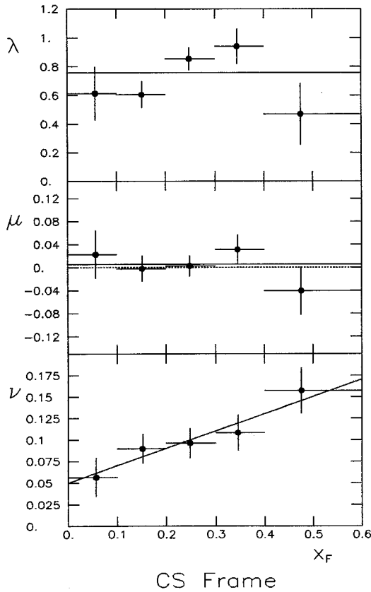
Fig. 8. Coefficients \lambda , \mu , and \nu as a function of x_F in the CS frame. The horizontal bars give the size of each interval. The solid lines represent the simple fits described in Sect. 4.4
