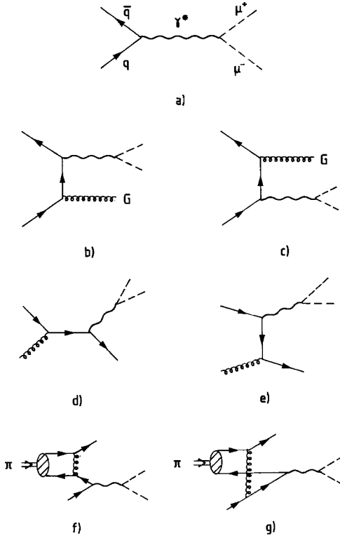
Fig. 1 a–g. Diagrams contributing to the Drell-Yan cross section; a: lowest order; b, c: first-order annihilation with gluon emission; d, e: first-order gluon Compton scattering; f, g: higher-twist contributions to the photon polarization
