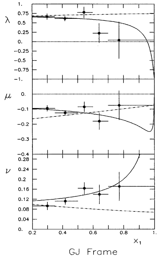
Fig. 9. Coefficients \lambda , \mu , and \nu as a function of x_1 in the GJ frame. The horizontal bars give the size of each interval. For \lambda and \mu the solid lines are the results of the simultaneous fit to (34) and (35) (higher-twist effect), and for \nu it is given by (15). The dot-dashed lines correspond to the leading-twist approximation, assuming \lambda and \nu constant and \mu=0 in the CS frame
