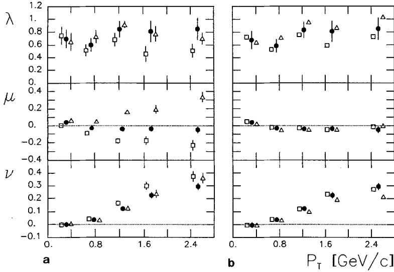
Fig. 4 a, b. Coefficients \lambda , \mu , and \nu as functions of P_T . a In the three different frames. Full circles: CS frame; open squares: GJ frame; open triangles: UC frame. b In the CS frame. Full circles: obtained in the CS frame; open squares: values from the GJ frame transformed to the CS frame; open triangles: values from the UC frame transformed to the CS frame. The squares and triangles are slightly displaced for clarity
