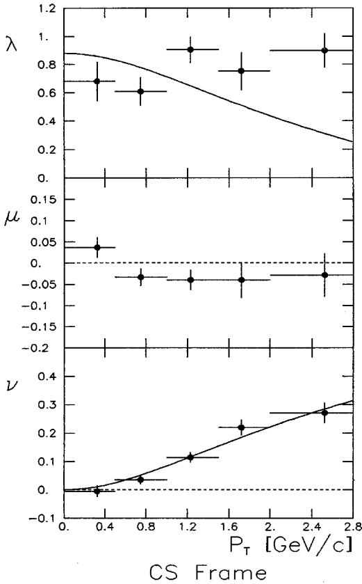
Fig. 6. Coefficients \lambda , \mu , and \nu as a function of P_T in the CS frame. The horizontal bars give the size of each interval. For \nu , the solid line is the result of the fit to (24), for \lambda it is given by (15)
