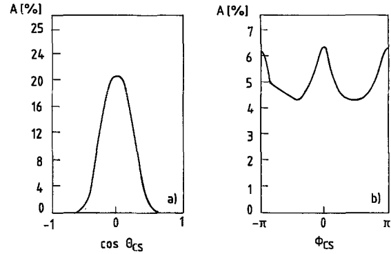
Fig. 3a, b. Spectrometer acceptance as a function of the two angular variables \cos \theta a, and \phi b, as computed by Monte-Carlo
