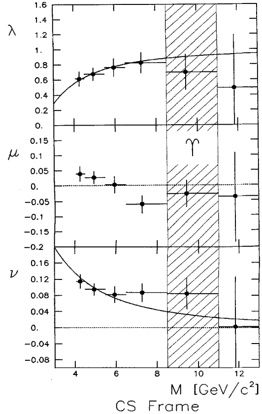
Fig. 5. Coefficients \lambda , \mu , and \nu as a function of M in the CS frame. The horizontal bars give the size of each interval. For \nu , the solid line corresponds to the fit to (24), and for \lambda to the fit to (13). The shaded interval corresponds to the \Upsilon region and is omitted in the fit
