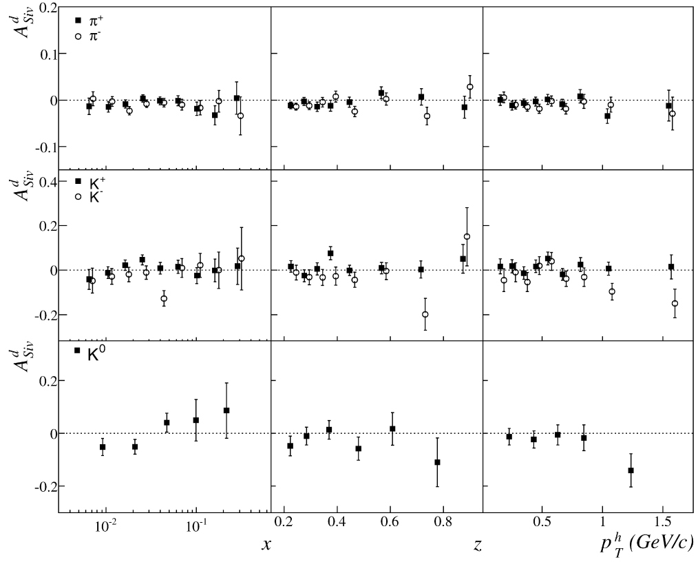
Fig. 7. Sivers asymmetry against x , z and p_T^h for the “all” charged pions and kaons samples from the 2003–2004 data, and “all” K_S^0 ’s sample from the 2002–2004 data.
