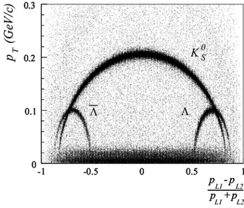
Fig. 4. Armenteros plot of the hadron pair. The K_S^0 band can be clearly seen as well as the \Lambda and \bar{\Lambda} bands.
