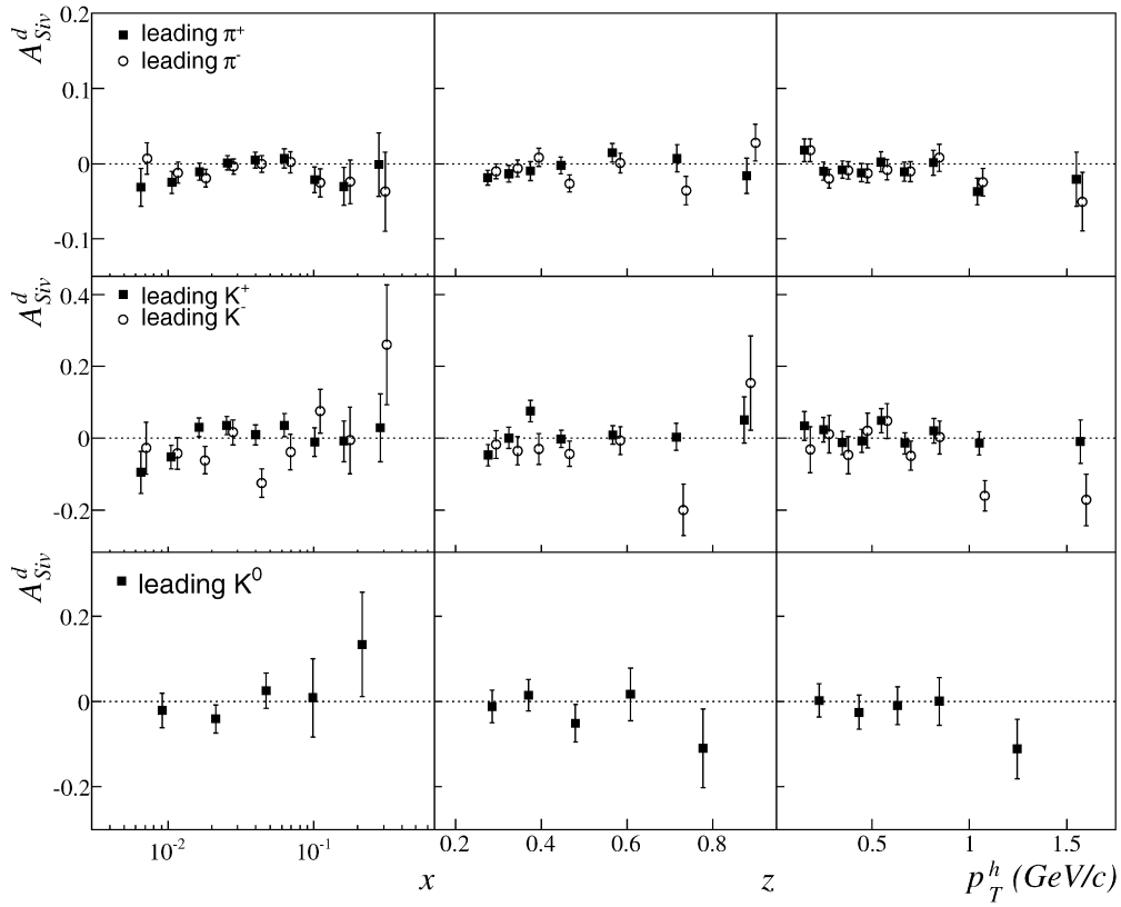
Fig. 9. Sivers asymmetry against x , z and p_T^h for the “leading” charged pions and kaons samples from the 2003–2004 data, and “leading” K_S^0 s sample from the 2002–2004 data.
