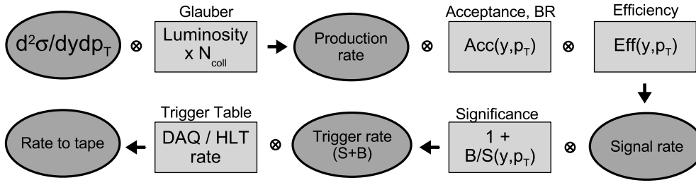
Figure 5.2. Schematic description of the HLT simulation chain. Input cross sections are obtained from PYTHIA 6.326 or NLO pQCD calculations. Acceptance, efficiency and background levels are parameterised from full GEANT4 based simulations. See the text for detailed descriptions of each of the steps.
