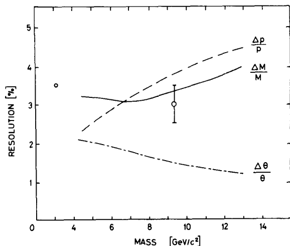
Fig. 9. Spectrometer resolution, as determined by Monte Carlo (curves) and by a fit to the data (circles).
