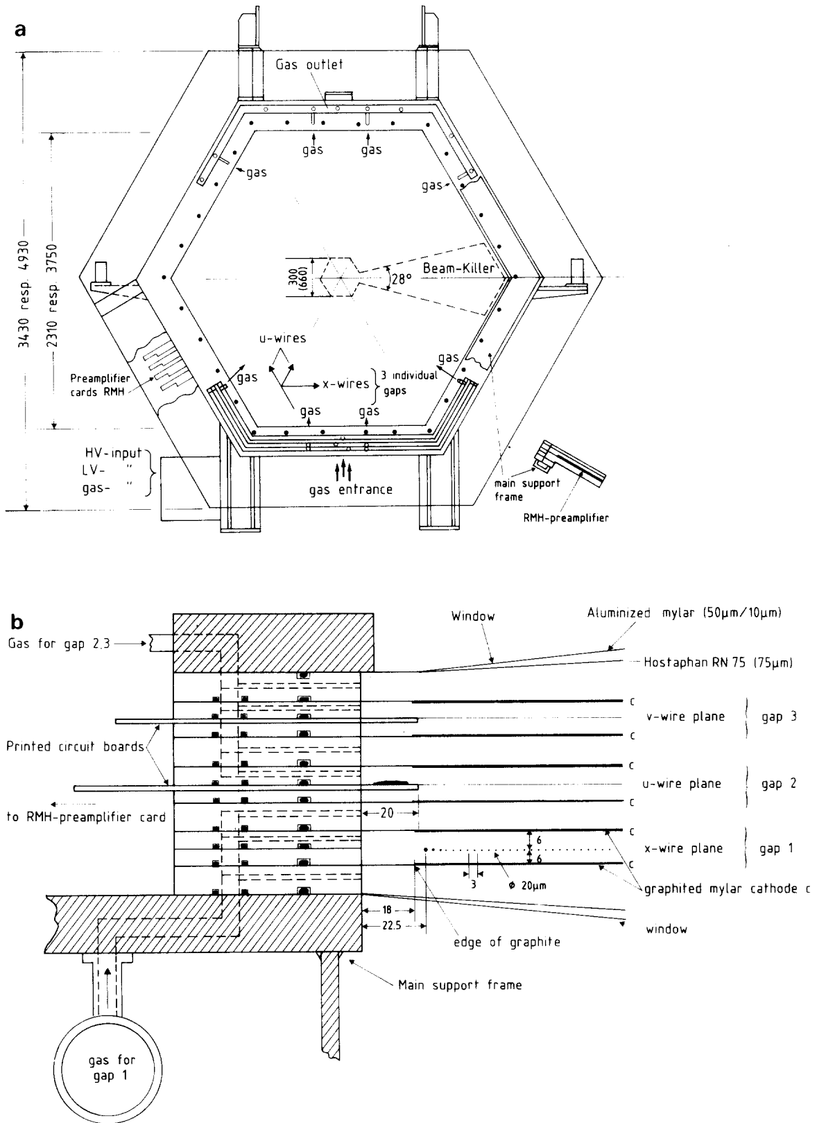
Fig. 2. MWPC design. (a) Front view of the chamber. (b) Cross section of chamber edge.
