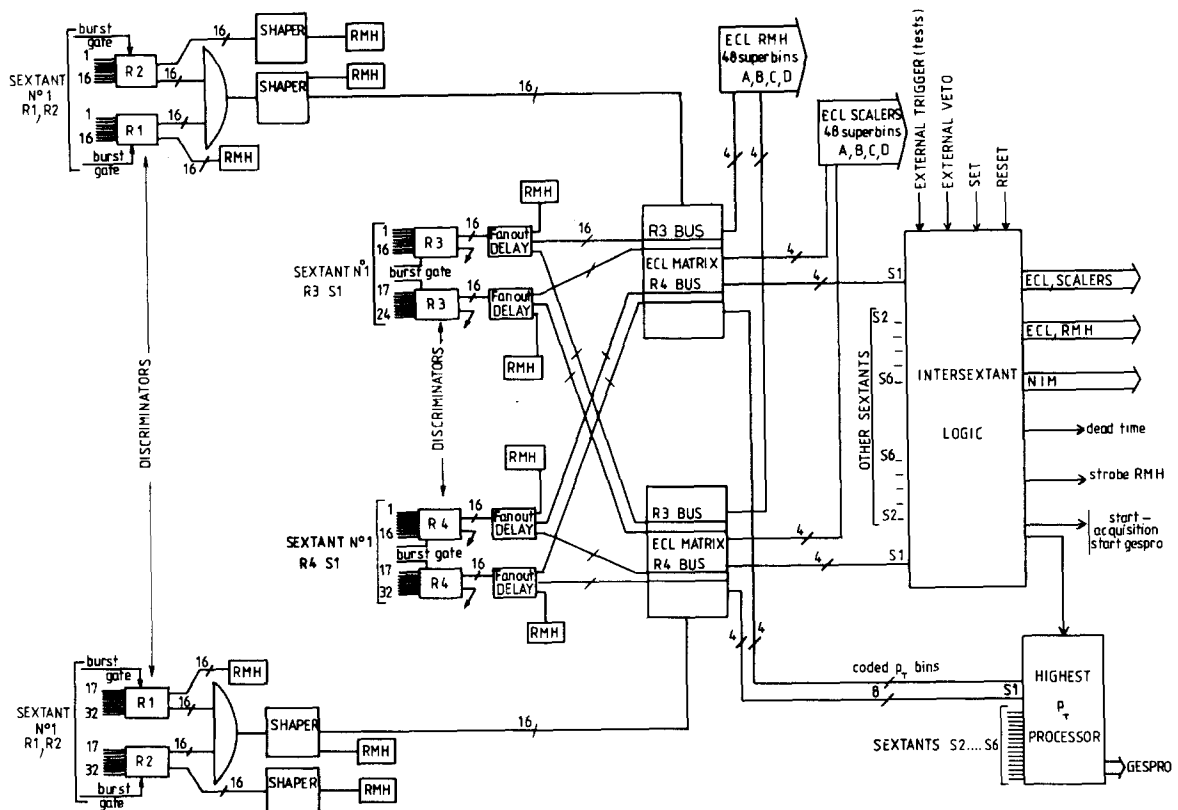
Fig. 5. Fast logic.
