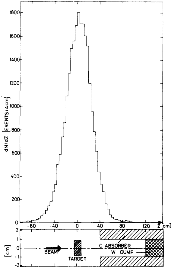
Fig. 7. Vertex distribution for a 12 cm tungsten target.
