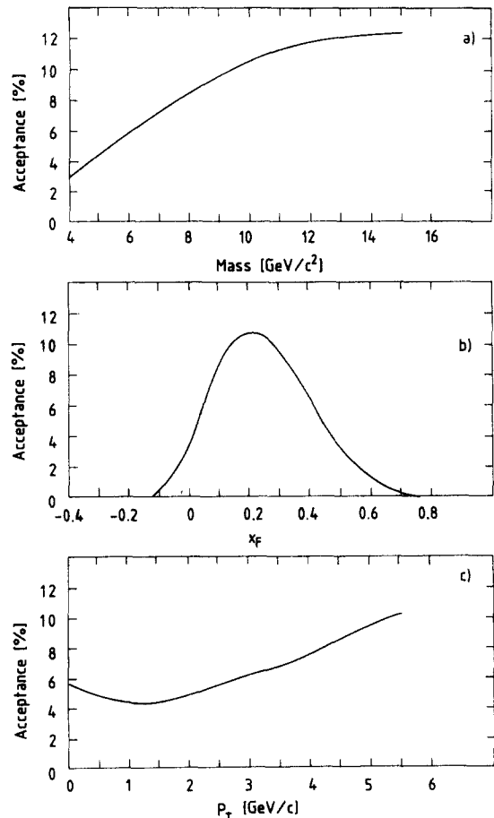
Fig. 8. Spectrometer acceptance: a) vs. dimuon mass M ; b) vs. Feynman x_F ; c) vs. transverse momentum P_T .
