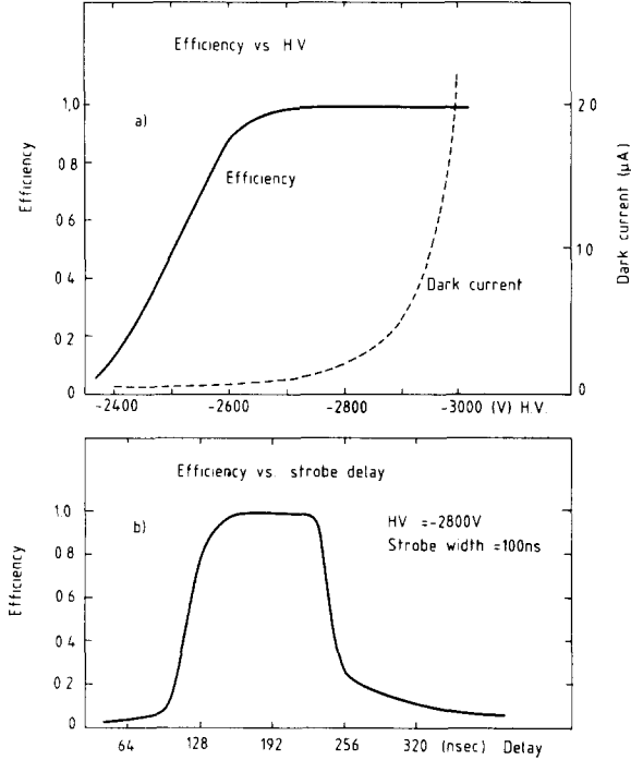
Fig. 3. MWPC plateau and delay curves.
