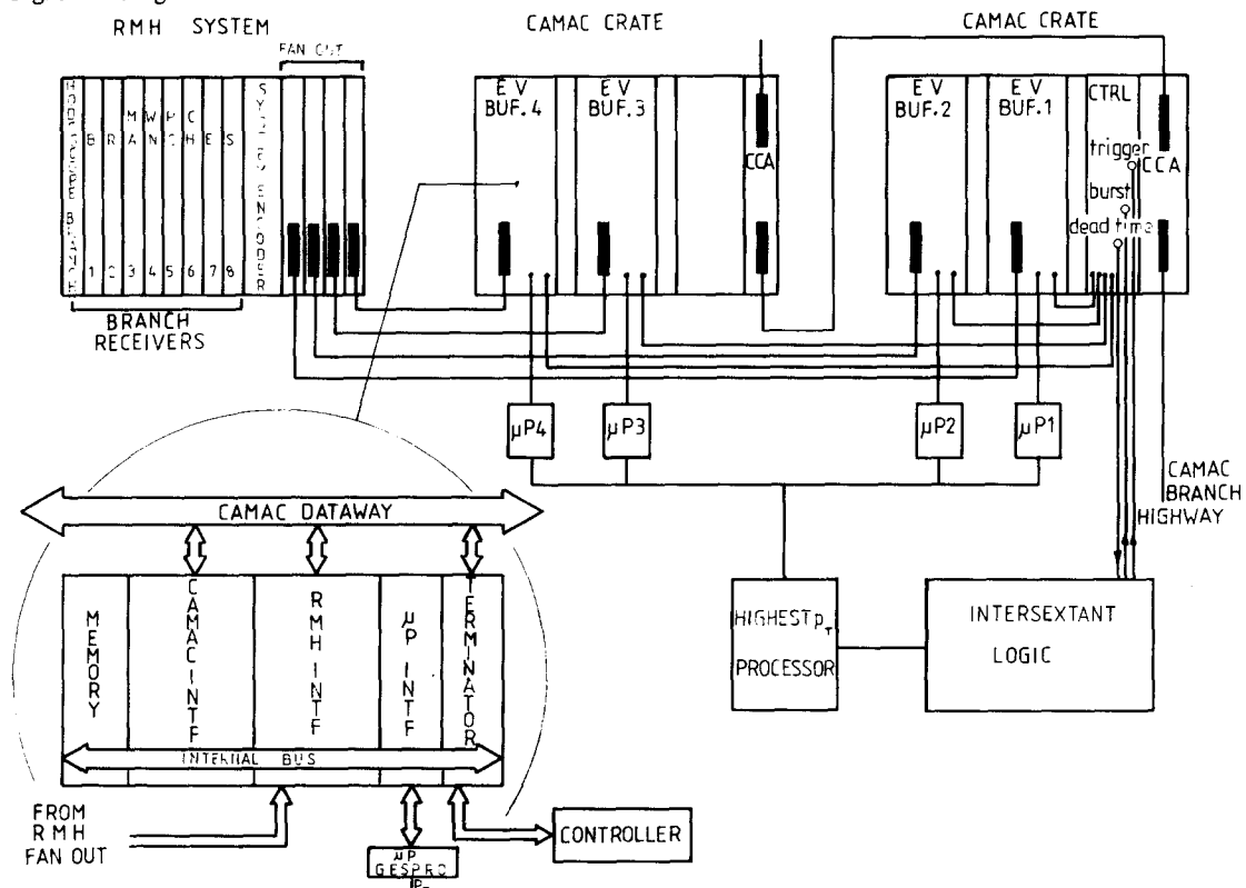
Fig. 6. Event-buffer/microprocessor system.
