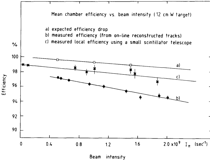
Fig. 4. MWPC efficiencies.
