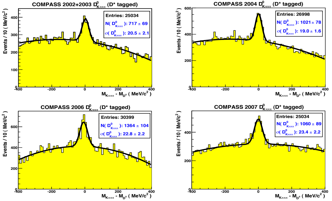
Figure 5.16: Invariant mass distributions of the D^*_{K\pi\pi\pi} channel.
