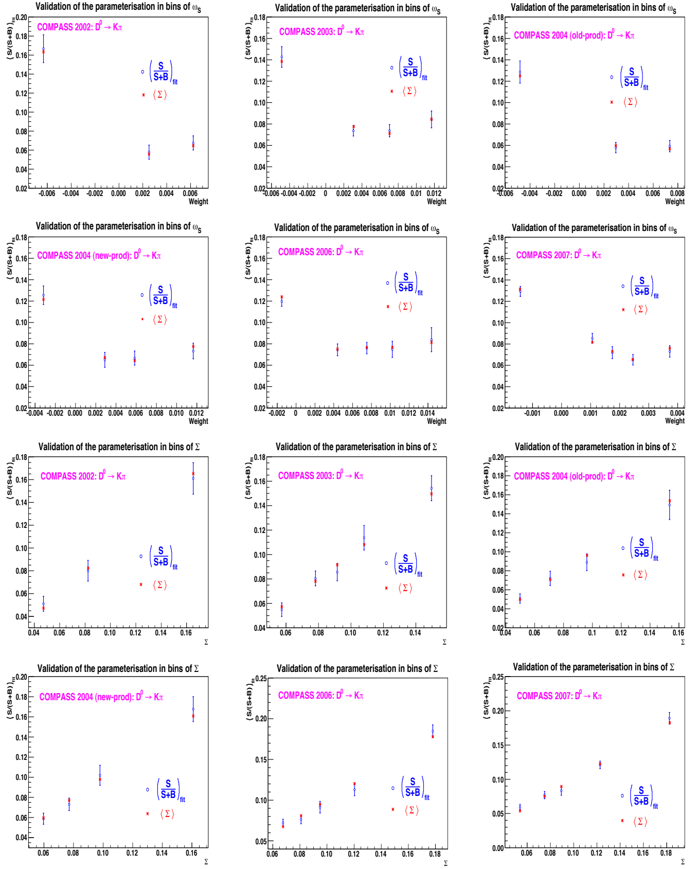
Figure 7.18: D^0_{K\pi} channel: validation of all parameterisations ( \Sigma_{19}, \Sigma_{20}, \Sigma_{21}, \Sigma_{22}, \Sigma_{23}, \Sigma_{24} ) in bins of weight (first 2 lines) and also in bins of probability (last 2 lines).
