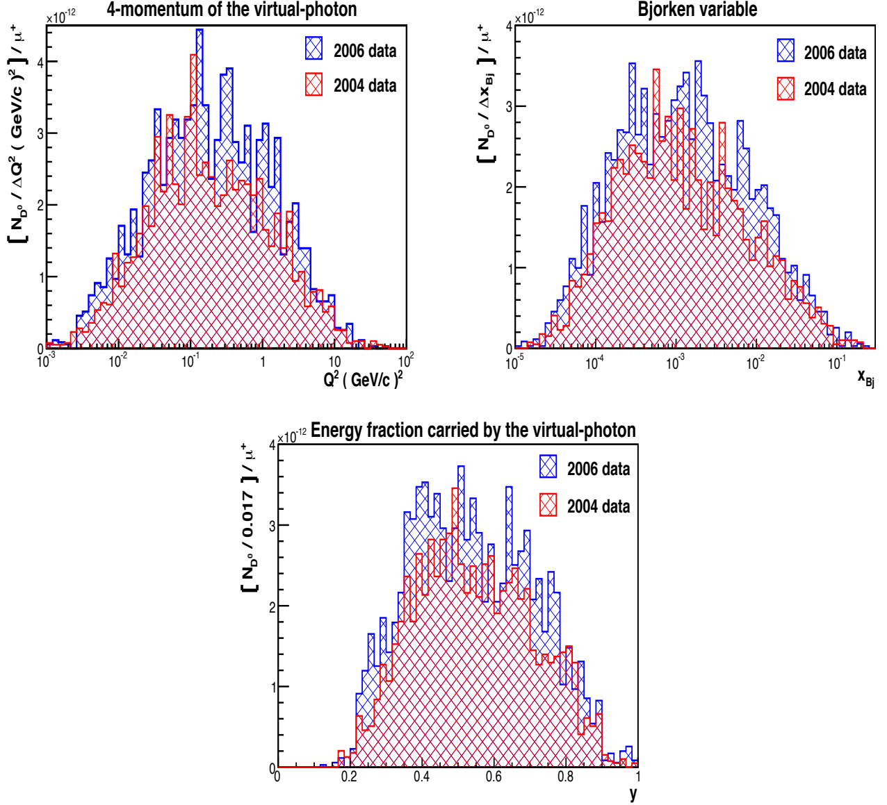
Figure 5.19: Distributions of the most important DIS variables obtained from the D_{K\pi}^* channel, using only D^0 candidates within a mass window of \pm 80 MeV/ c^2 . Note that the x_{Bj} distribution is limited to the interval defined by x_{Bj} < 0.1 . The latter is a strong support to the assumption of no intrinsic-charm in the nucleon for the present analysis.
