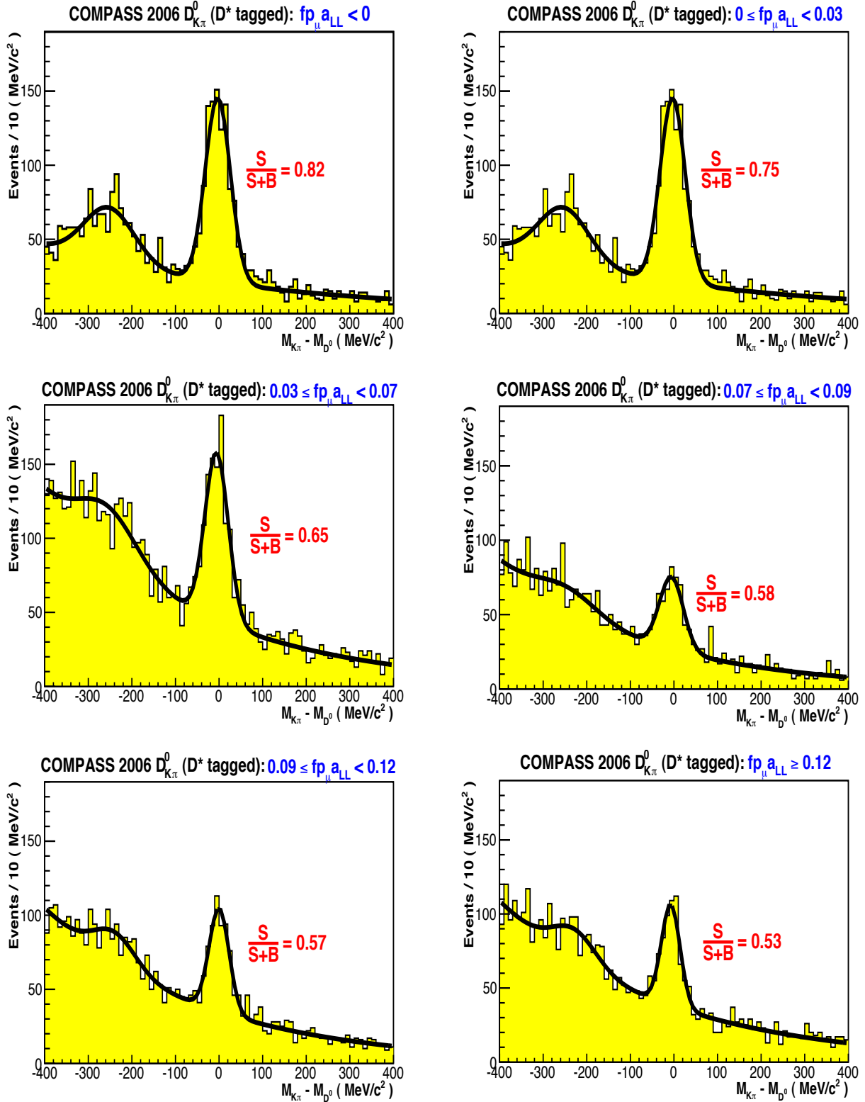
Figure 7.11: D^{*0}_{K\pi} (2006) sample in bins of fP_\mu a_{LL} . The anti-correlation between S/(S+B) and the remaining part of the event weight is clear (these signal purities are obtained from a fit to the mass spectra in a window of \pm 40 \text{ MeV}/c^2 ).
