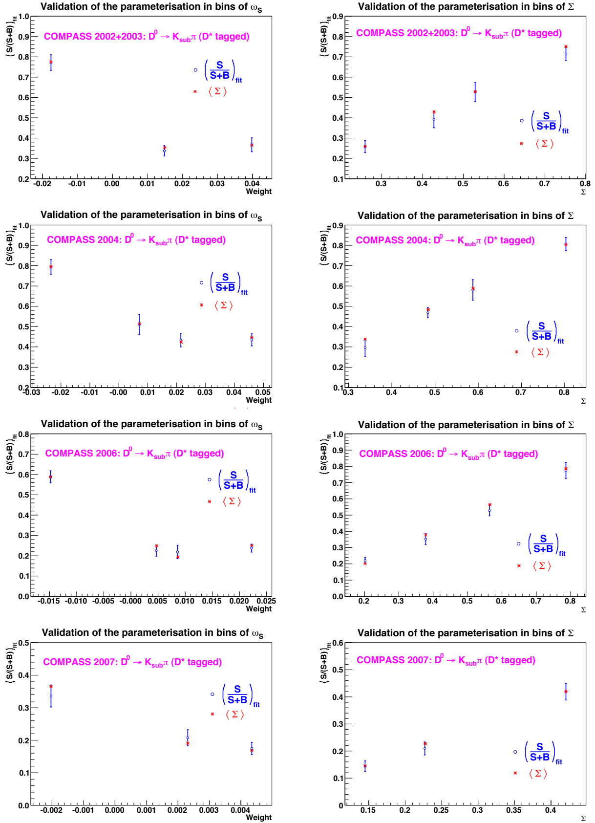
Figure 7.20: D^0_{K_{sub}\pi} channel: validation of all parameterisations ( \Sigma_{15} , \Sigma_{16} , \Sigma_{17} , \Sigma_{18} ) in bins of weight (first column) and also in bins of probability (second column).
