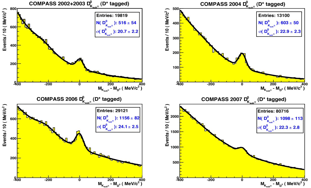
Figure 5.17: Invariant mass distributions of the D^*_{K_{sub\pi\pi}\pi} channel.
