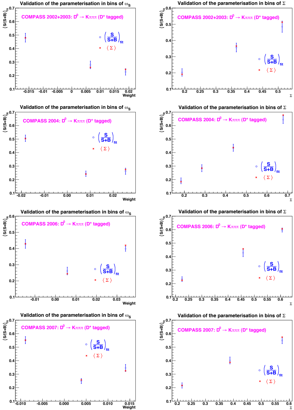
Figure 7.19: D^0_{K\pi\pi\pi} channel: validation of all parameterisations ( \Sigma_{11} , \Sigma_{12} , \Sigma_{13} , \Sigma_{14} ) in bins of weight (first column) and also in bins of probability (second column).
