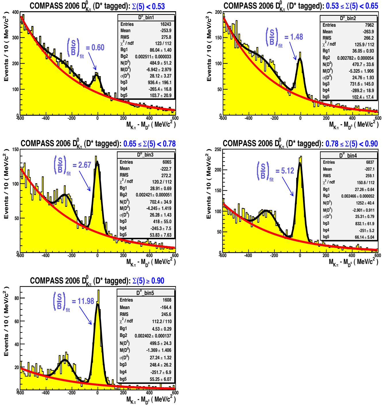
Figure 7.23: D_{K\pi}^0 (2006) mass spectrum in bins of D^0 probability ( \Sigma ). The fits shown are used to introduce the mass dependence in \Sigma(5) and also to validate the parameterisation (11 th plot in Fig. 7.17)
