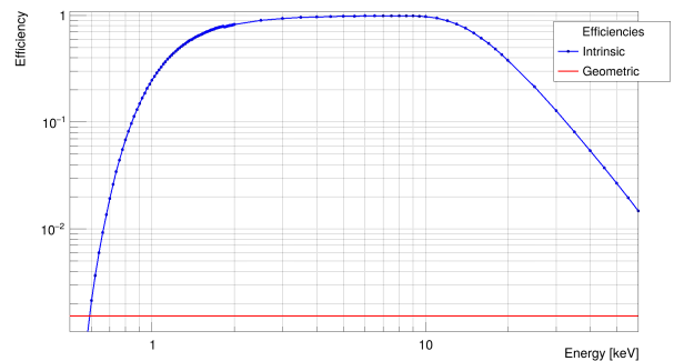
Figure 16: Detector efficiencies. The blue curve shows the intrinsic efficiency. The red line shows the theoretical value for the geometrical efficiency.
