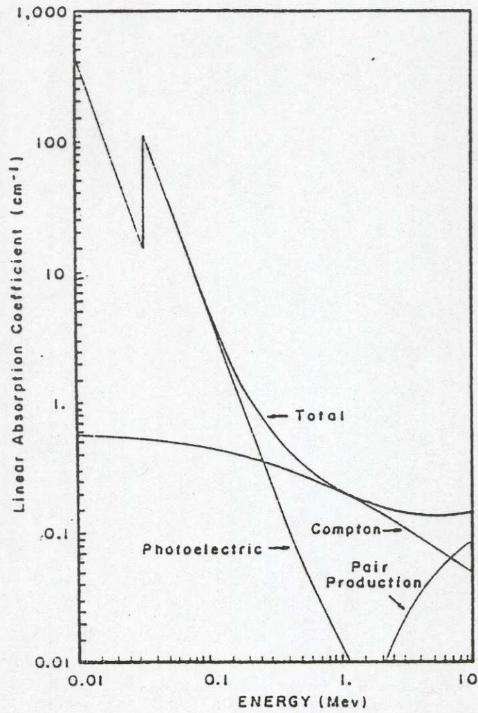
Figure 2-21. Variation of photoelectric, Compton, pair production, and total cross sections for sodium iodide as a function of energy.
