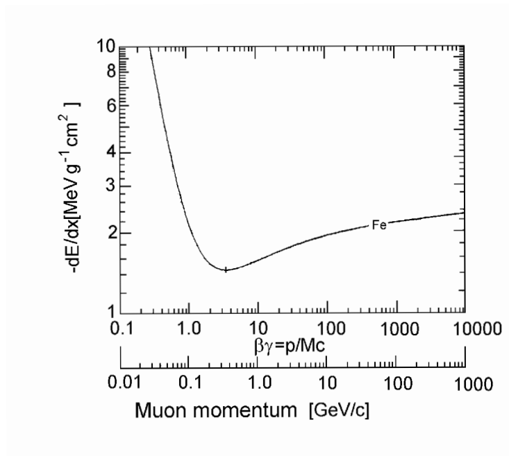
FIGURE 4. Energy loss of muons in iron [6]
