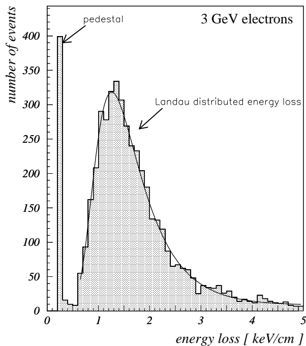
FIGURE 6. Energy-loss distribution of 3 GeV electrons in a thin-gap multiwire drift chamber [13]
