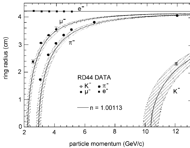
FIGURE 9. Cherenkov-ring radii of e , \mu , \pi , K in a C_4F_{10} -Ar (75:25) RICH-counter. The solid curves show the expected radii for an index of refraction of n = 1.00113 . The shaded regions represent a 5% uncertainty in the absolute momentum scale [17]
