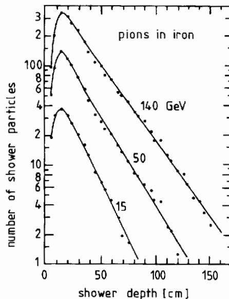
FIGURE 17. Longitudinal development of pion induced hadron cascades [25]
