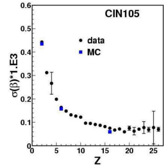
Figure 6. Velocity accuracy dependence on the charge.
