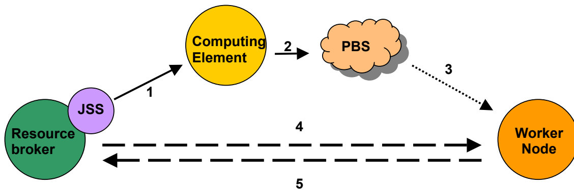
Figure 10 – job submission and sandboxes transfer
