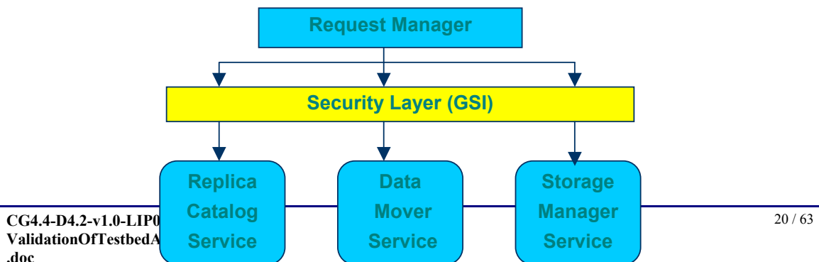
Figure 12 – GDMP architecture
